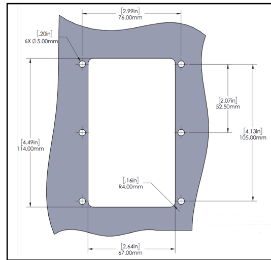
Figure 3.1.1: i-AVT-N Plus cutout dimensions.
