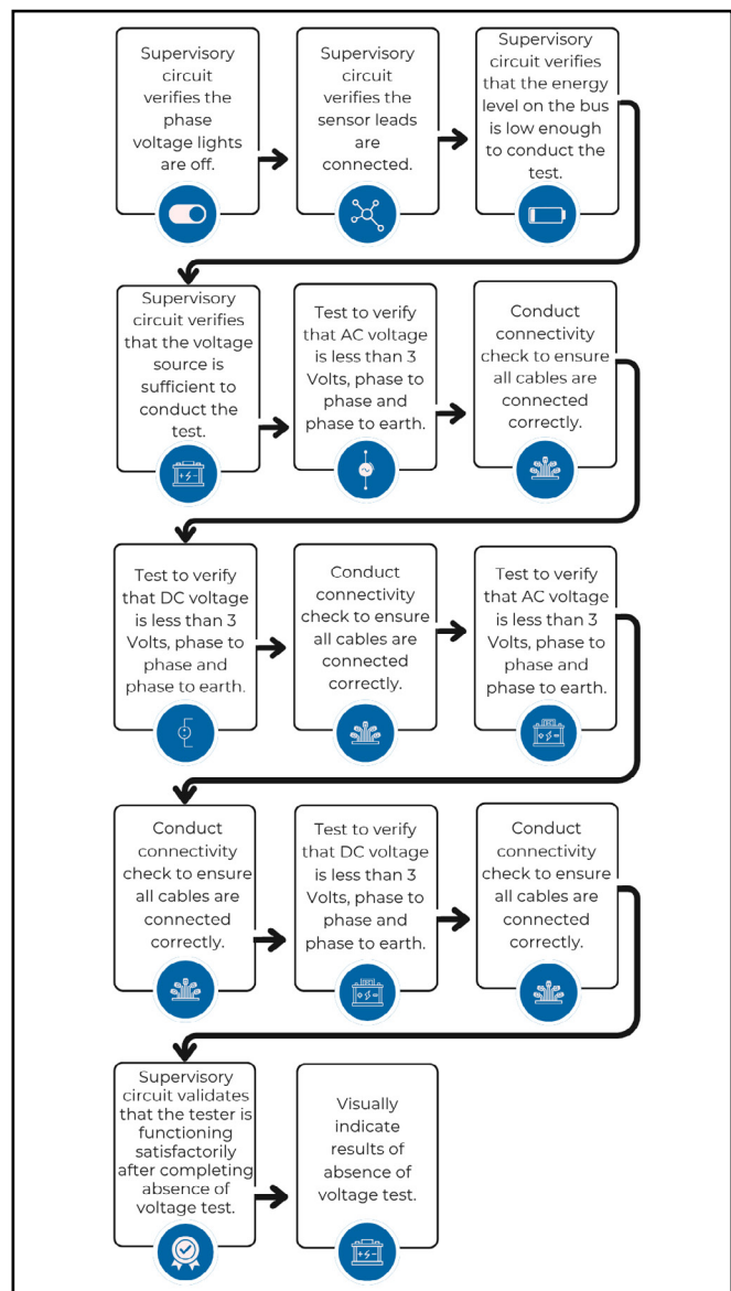
Figure 5.5: Flowchart for determining Absence of Voltage
