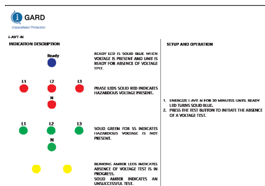
Figure 2.2: i-AVT-N Label
