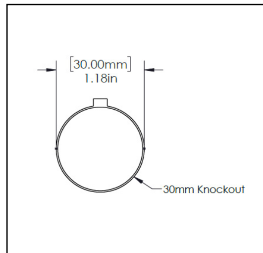
Figure 3.1.1: i-AVT-N cutout dimensions.
