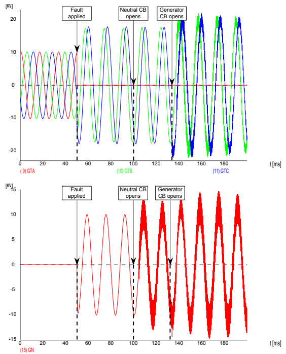
Figure 9. Generator terminal voltage (top) and neutral voltage (bottom) for Case 1b - Neutral breaker opens in 3 cycles and the main breaker opens in 5 cycles (cable pi-equivalent plus current chop)
