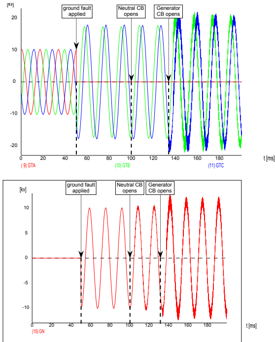
Figure 8. Generator terminal voltage (top) and neutral voltage (bottom) for Case 1a - Neutral breaker opens in 3 cycles and the main breaker opens in 5 cycles (cable pi-equivalent)
