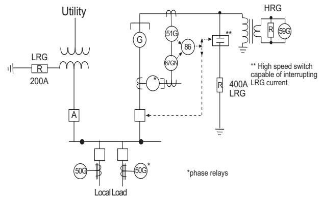
Figure 5. Hybrid Grounded and Associated Ground Fault Protection
