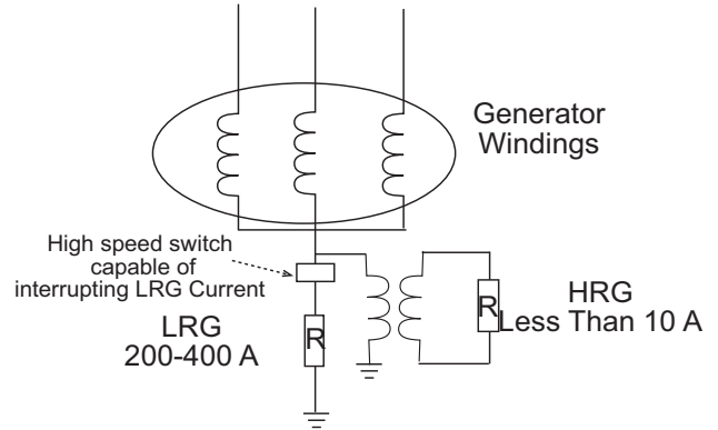
Figure 4. Generator Hybrid Ground
