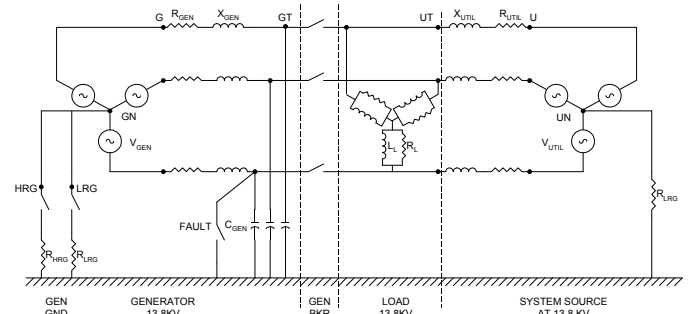
Figure 7. Initial System Model for EMTP Simulations
