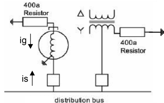
Figure 1. Medium-Voltage Industrial Distribution System with Multiple Sources
