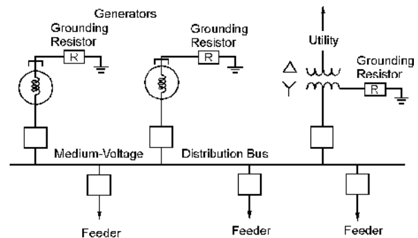
Figure 1. Medium-Voltage Industrial Distribution System with Multiple Sources
