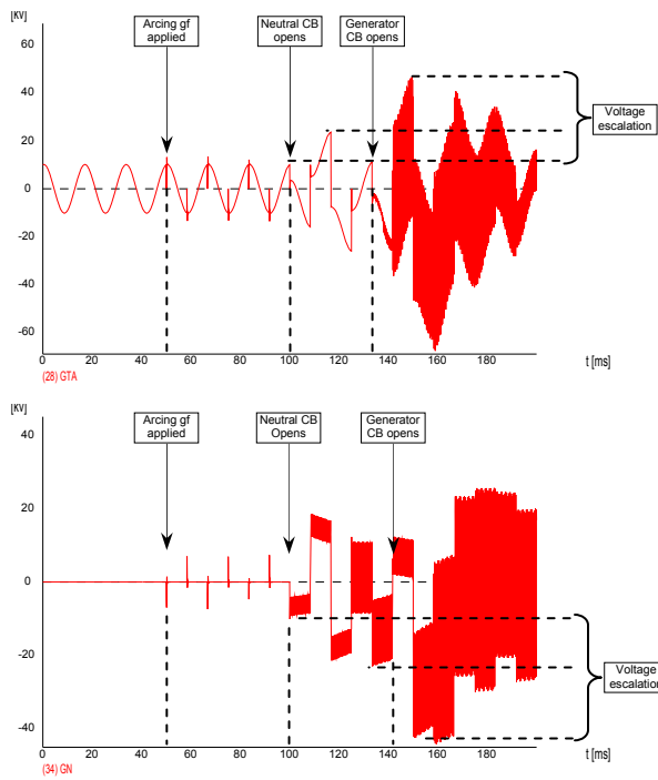
Figure 11. Generator terminal voltage (top) and neutral voltage (bottom) for Case 6-generator ungrounded - Neutral breaker opens in 3 cycles and the main breaker opens in 5 cycles (arcig ground fault on phase-A)
