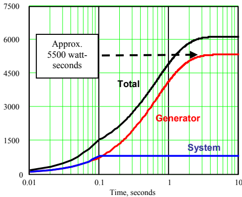
Figure 3. Watt-Second Fault Energy vs. Time
