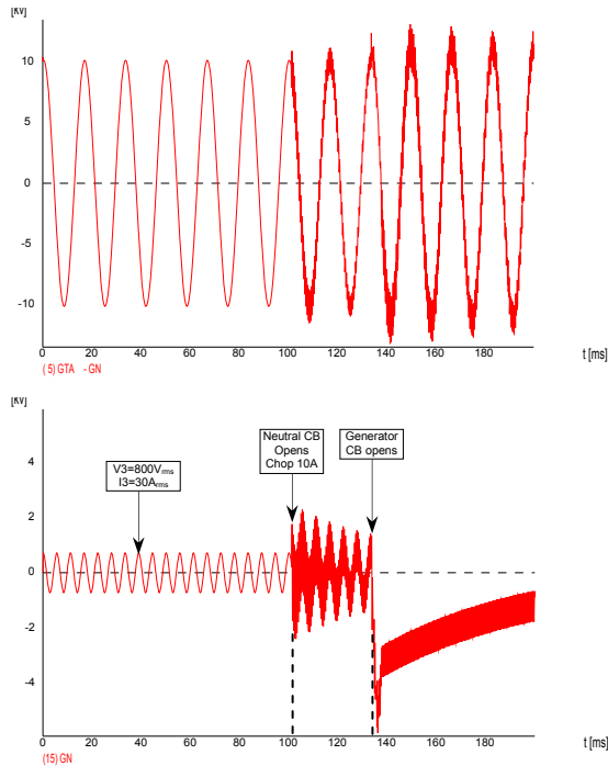
Figure 10. Generator terminal voltage (top) and neutral voltage (bottom) for Case 4 - Neutral breaker opens in 3 cycles and the main breaker opens in 5 cycles (chop at 10 A of 3 rd harmonic current)
