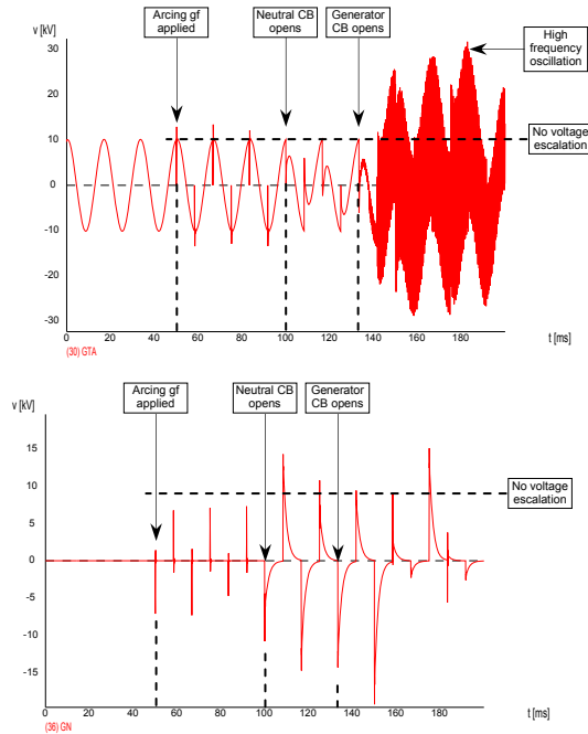
Figure 13 Generator terminal voltage (top) and neutral voltage (bottom) for Case 7b with HRG component and arcing ground fault at 50 msec and internal voltage decay ( T_{ig} of 1.0).
