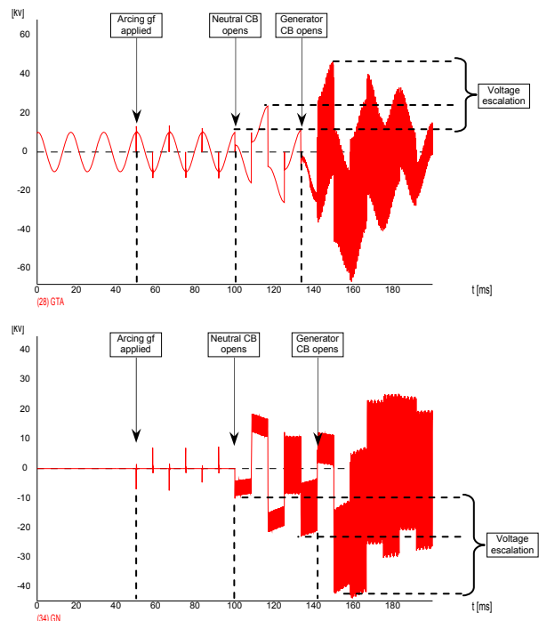
Figure 12. Generator terminal voltage (top) and neutral voltage (bottom) for Case 6b (generator ungrounded) arcing ground fault at 50 msec and internal voltage decay ( T_{lg} of 1.0)
