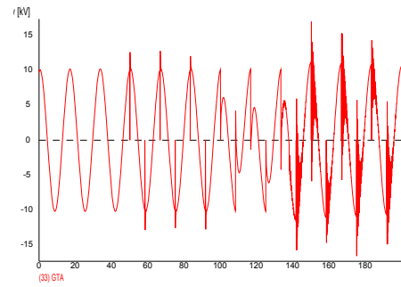
Fig 14 Generator terminal voltage for case 7g – added line terminal snubbers to case 7b
